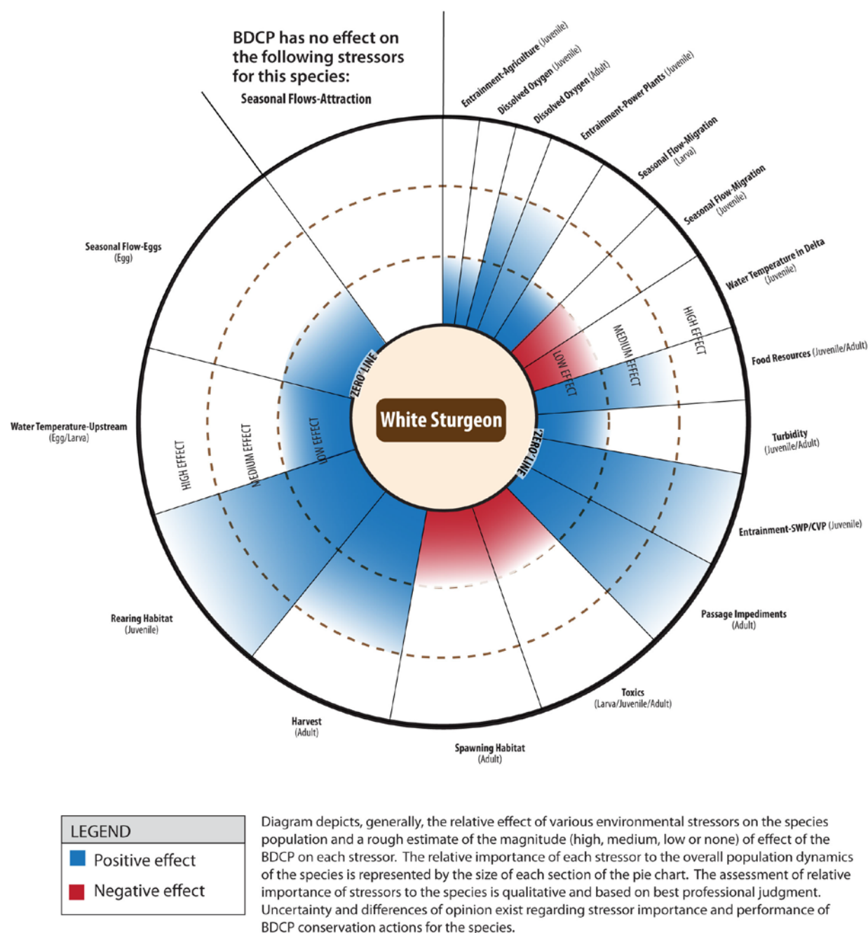
Figure 5-741. Population Level Effects by Stressors – White Sturgeon
