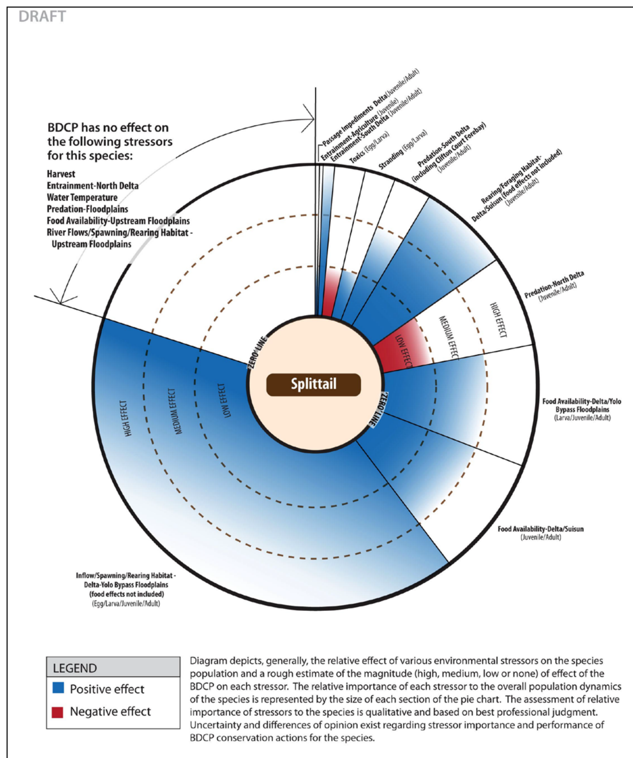
Figure 5-643. Population Level Effects by Stressors - Splittail
