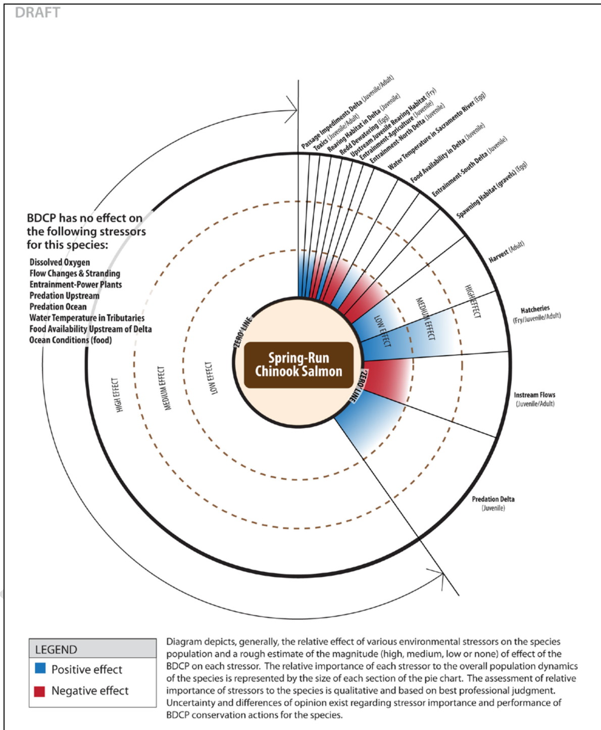
Figure 5-445. Population Level Effects by Stressors – Spring-Run Chinook Salmon
