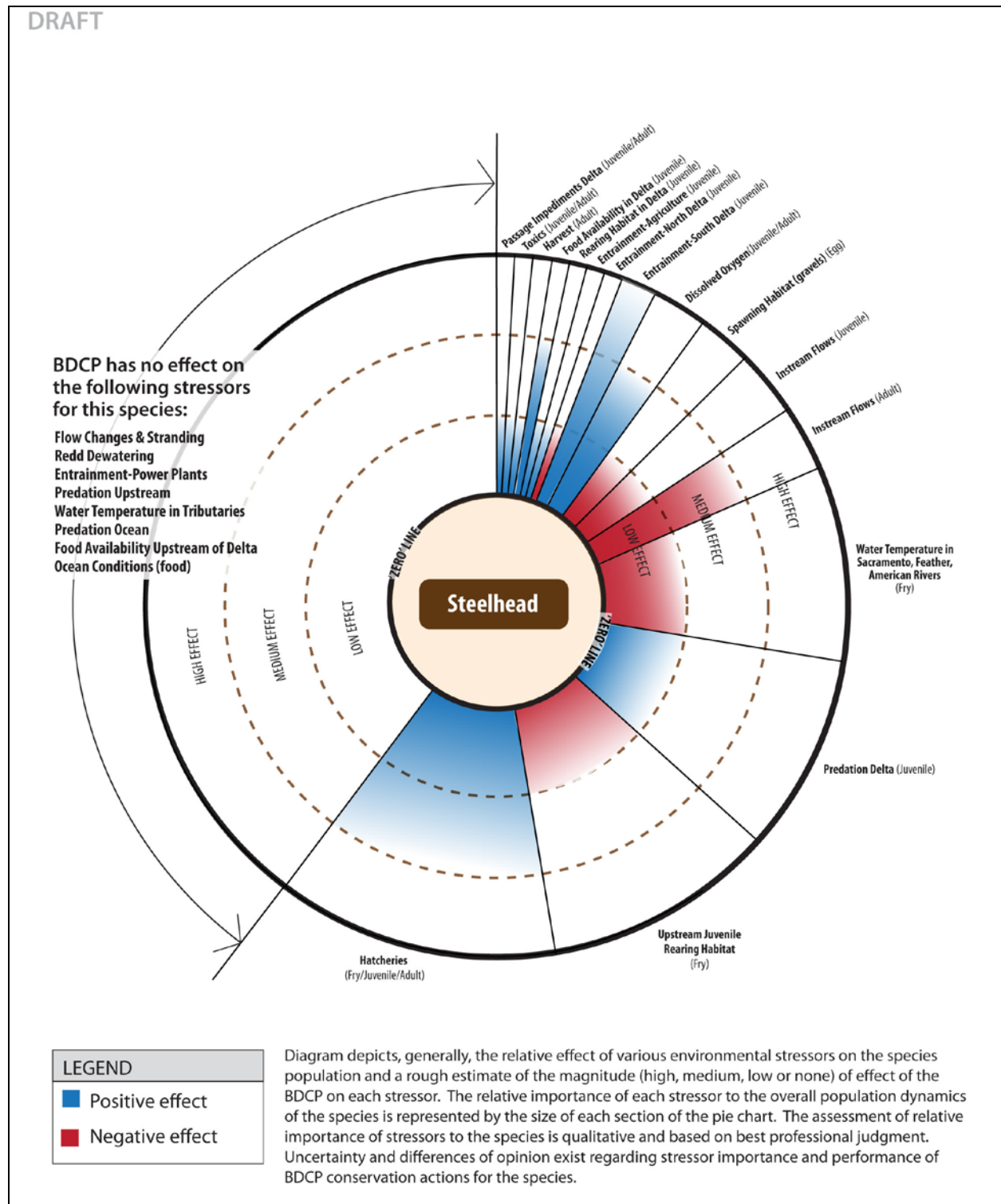
Figure 5-304. Population Level Effects by Stressors - Steelhead
