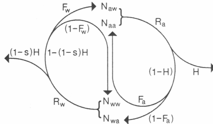
Figure 3, life cycle schematic, including hatchery production and harvest. N_{xy} is the number of spawner of origin y in habitat x , where w is natural and a is hatchery. R_y are the recruits, and F_y are the fractions of the natural and hatchery recruits taken into the hatchery. H is harvest, and s is the harvest selectivity for hatchery fish. Modified from Goodman (2004)
